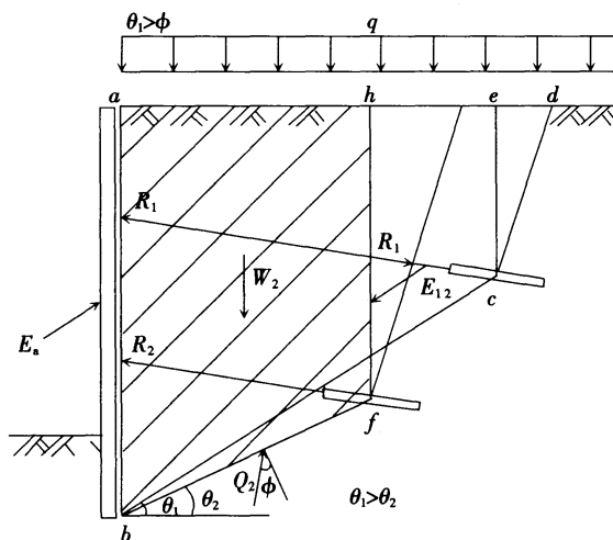
(a) 力系平衡
